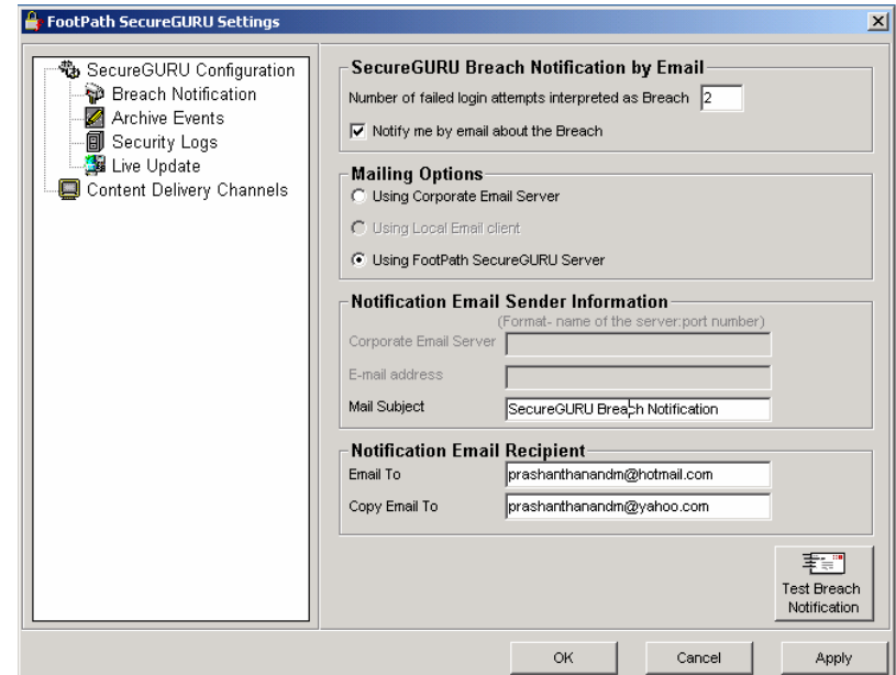
SecureGURU Configuration Panel
